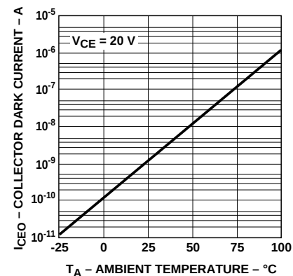
Figure 9. Collector dark current vs. temperature.
