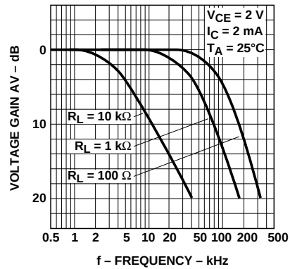
Figure 11. Frequency response.
