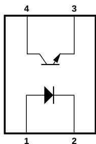
PIN NO. AND INTERNAL CONNECTION DIAGRAM
